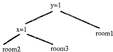
Figure 5. The Corresponding Tree Data Structure for Figure 4. Interior Nodes Represent Splitting Planes and Leaf Nodes Represent Cell Volumes.
